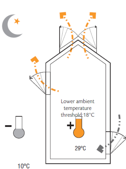
Night-cooling
